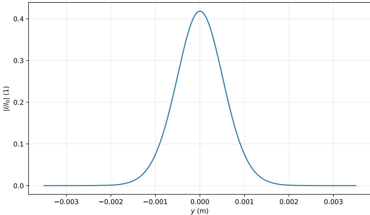
Intensity profile I(x=0, y, z=3.025)/I_0 , P_{in}=0.3P_{cr} , artificial time
